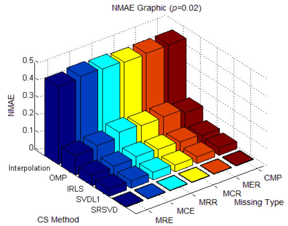
(a). Missing probability ( p=0.02 )
