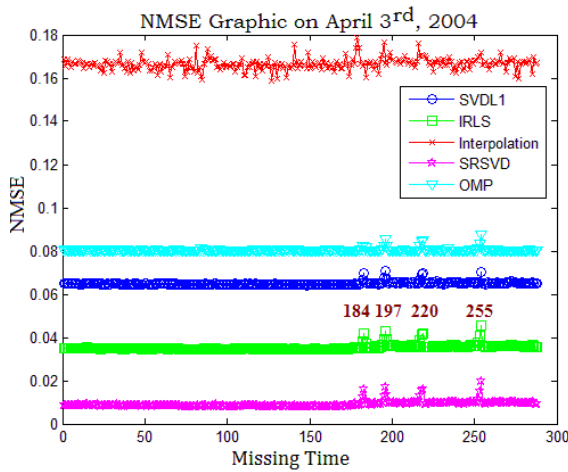
(b). NMSE on April 3 rd , 2004
