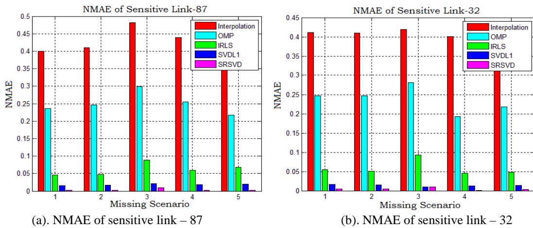
Figure 8. Missing scenario for tracing sensitive link composed, (a) NMAE of sensitive link number 87, (b) NMAE of sensitive link number 32
