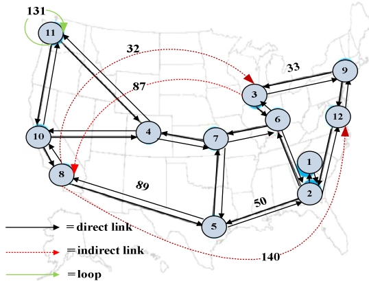
Figure 6. Representation of link connection
