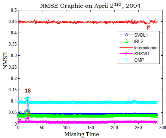
(a). NMSE on April 2 nd , 2004
