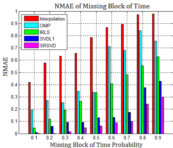
Figure 10. The missing block of time simulation
