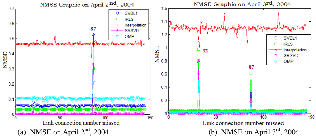
Figure 7. Detection of link sensitivity for a particular day, (a). NMSE on April 2 nd , 2004, (b). NMSE on April 3 rd , 2004
