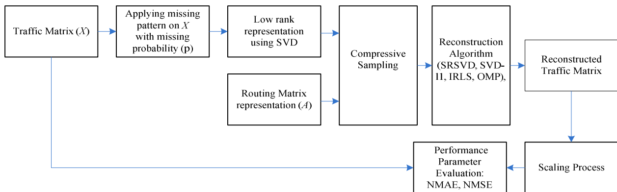
Figure 3. Missing internet traffic reconstruction processing using compressive sampling
